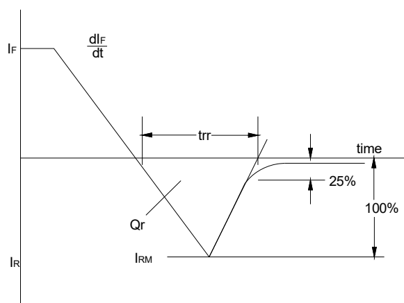
FIG.5: Reverse recovery definitions
