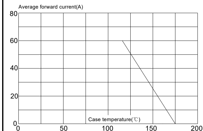
FIG.5 Forward current derating curve (Pin1,3~2)
