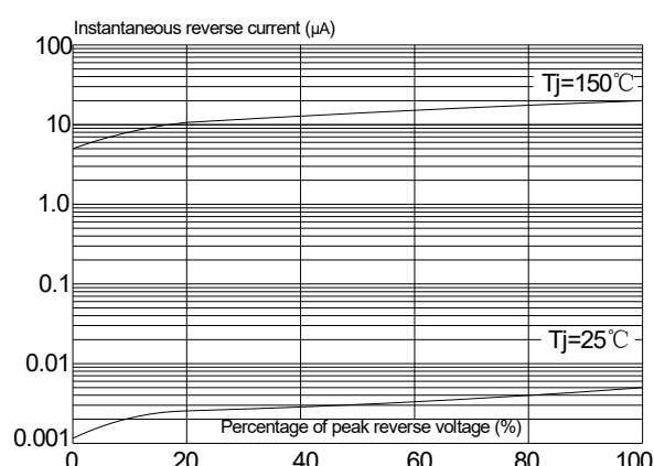
FIG.2: Typical reverse characteristics (Pin1~2 or Pin3~2)
