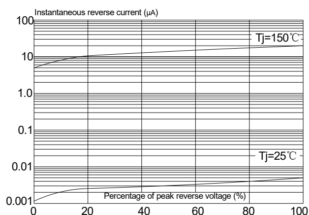
FIG.2: Typical reverse characteristics (Pin1~2 or Pin3~2)
