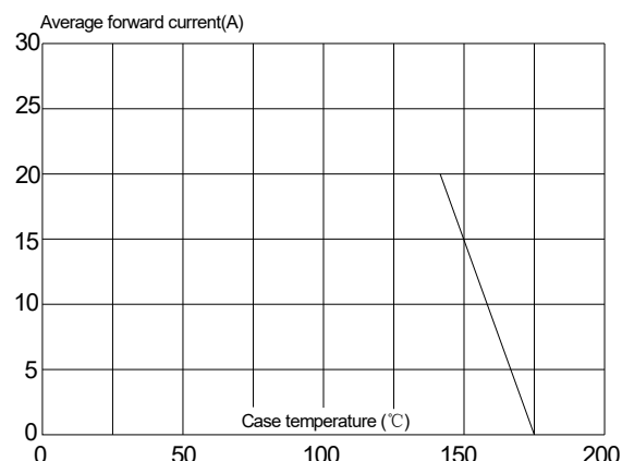
FIG.4: Forward current derating curve (Pin1,3~2)
