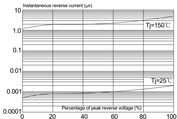
FIG.2: Typical reverse characteristics (Pin1~2 or Pin3~2)
