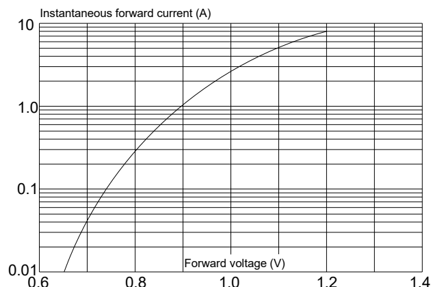
FIG.1: Typical forward characteristics(25°C)
