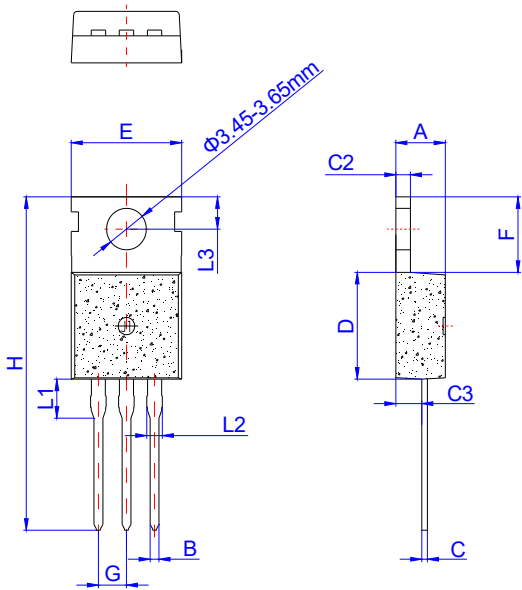
TO-220C
