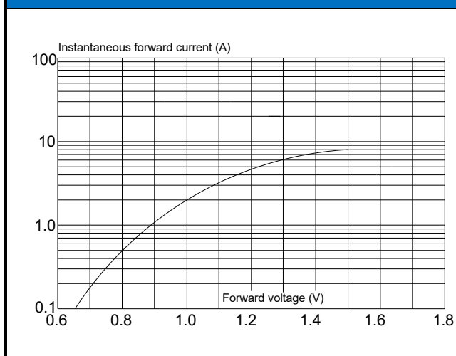
FIG.1: Typical forward characteristics(25°C)
