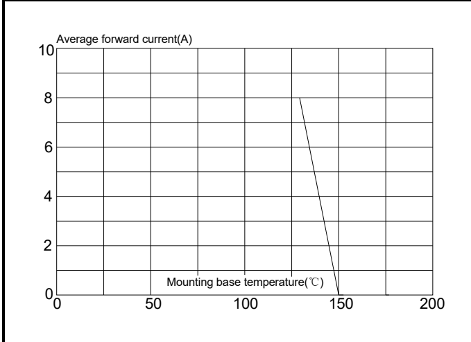
FIG.5: Forward current derating curve
