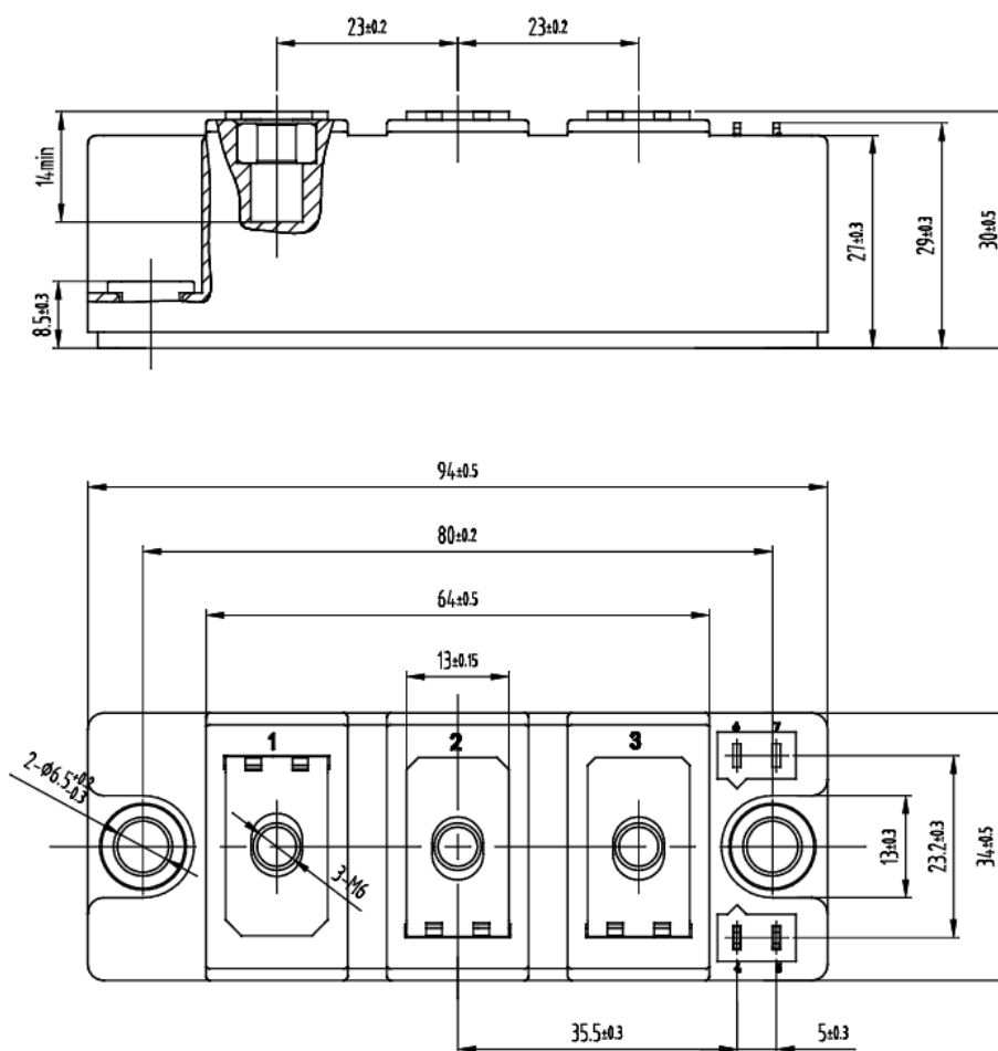
Package Outlines (mm)
