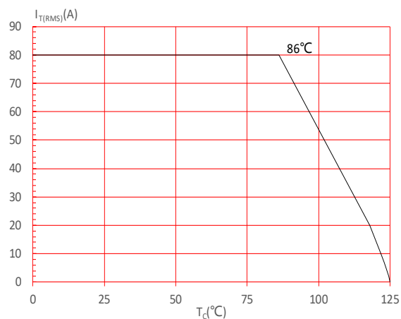
FIG.4: On-state characteristic
