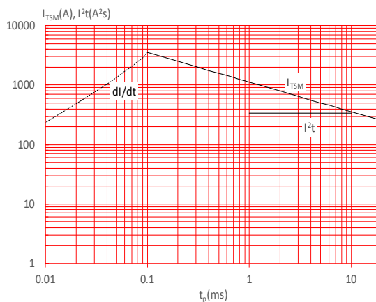
FIG.6: Non-repetitive surge peak on-state current for a sinusoidal pulse with width t_p < 20ms , and corresponding value of I^2t ( dl/dt < 100A/\mu s )
