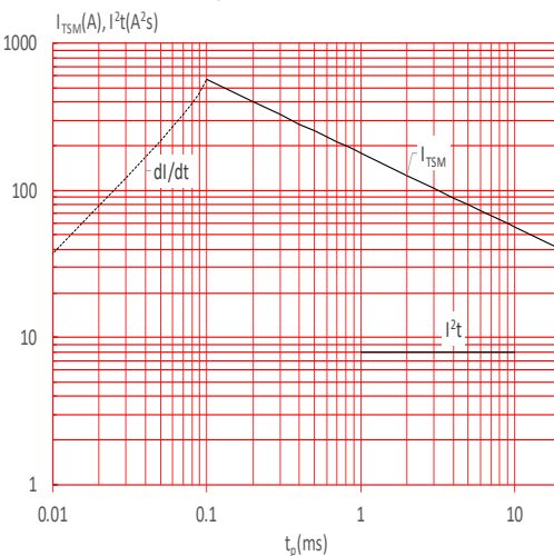
FIG.6: Non-repetitive surge peak on-state current for a sinusoidal pulse with width t_p < 20ms , and corresponding value of I^2t ( di/dt < 100A/\mu s )
