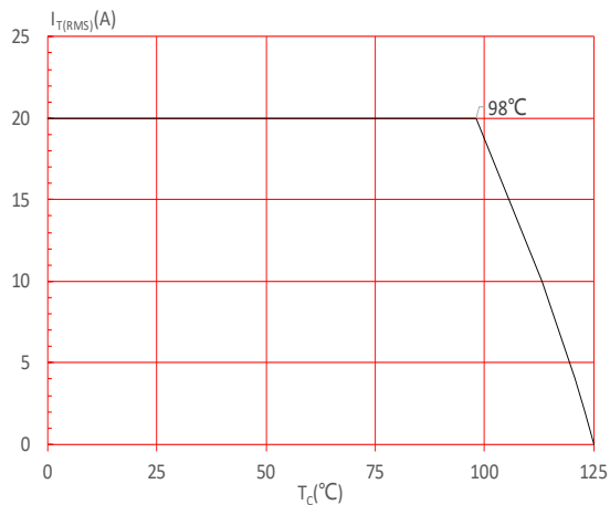
FIG.4: On-state characteristics
