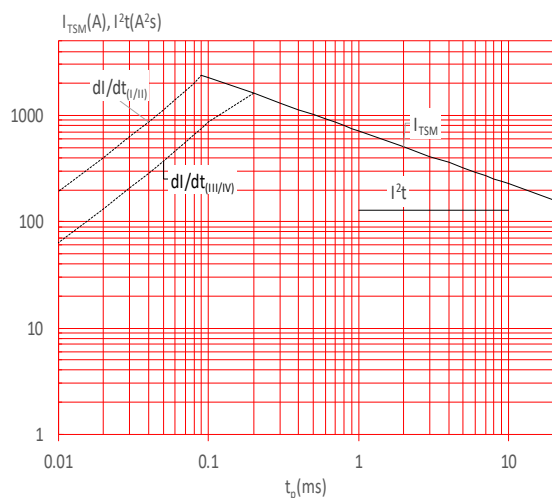
FIG.5: Non-repetitive surge peak on-state current for a sinusoidal pulse with width t_p < 20\text{ms} , and corresponding value of I^2t (I - II: di/dt < 100\text{A}/\mu\text{s} ; III-IV: di/dt < 50\text{A}/\mu\text{s} )
