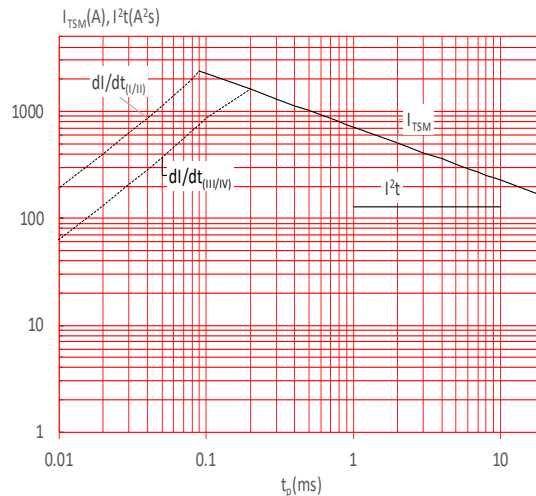
FIG.6: Non-repetitive surge peak on-state current for a sinusoidal pulse with width t_p < 20ms , and corresponding value of I^2t ( I - II: di/dt < 80A/\mu s ; III-IV: di/dt < 40A/\mu s )
