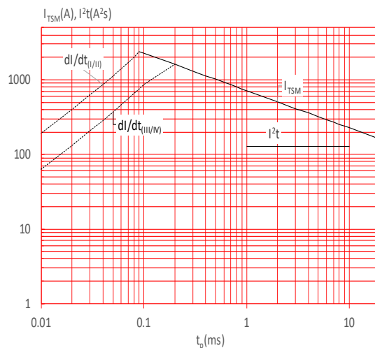
FIG.6: Non-repetitive surge peak on-state current for a sinusoidal pulse with width t_p < 20\text{ms} , and corresponding value of I^2t (I - II: dl/dt < 100\text{A}/\mu\text{s} ; III-IV: dl/dt < 50\text{A}/\mu\text{s} )
