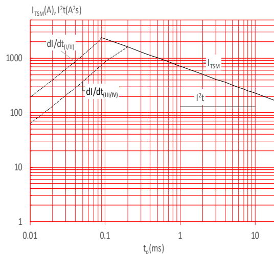
FIG.6: Non-repetitive surge peak on-state current for a sinusoidal pulse with width t_p < 20\text{ms} , and corresponding value of I^2t (I - II: dl/dt < 80\text{A}/\mu\text{s} ; III-IV: dl/dt < 40\text{A}/\mu\text{s} )
