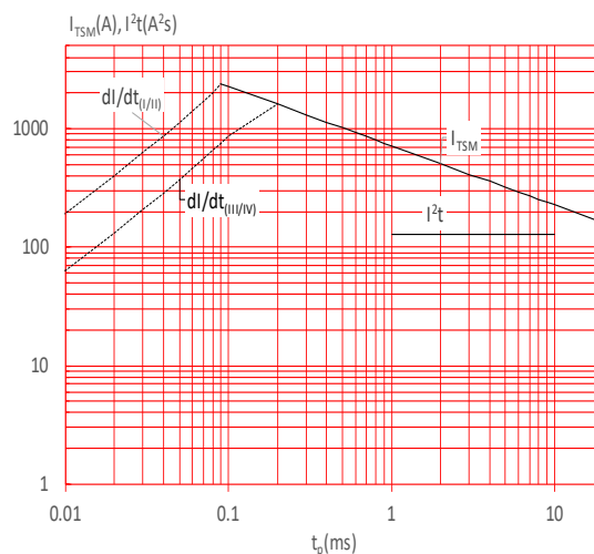
FIG.6: Non-repetitive surge peak on-state current for a sinusoidal pulse with width t_p < 20 ms, and corresponding value of I^2t (I - II: dl/dt < 100 A/ \mu s; III-IV: dl/dt < 50 A/ \mu s)
