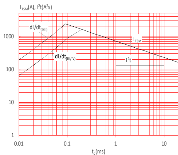
FIG.5: Non-repetitive surge peak on-state current for a sinusoidal pulse with width t_p < 20\text{ms} , and corresponding value of I^2t (I - II : di/dt < 80\text{A}/\mu\text{s} ; III-IV : di/dt < 40\text{A}/\mu\text{s} )
