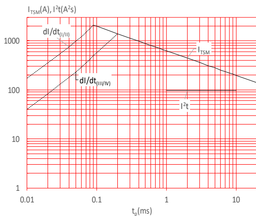
FIG.5: Non-repetitive surge peak on-state current for a sinusoidal pulse with width t_p < 20ms , and corresponding value of I^2t ( I - II : dl/dt < 100A/\mu s ; III-IV : dl/dt < 70A/\mu s )
