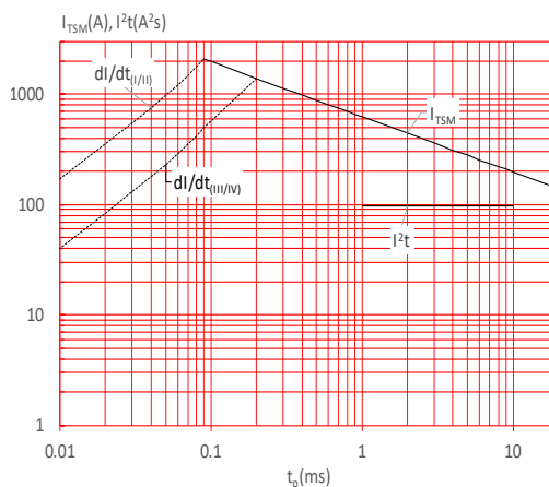
FIG.6: Non-repetitive surge peak on-state current for a sinusoidal pulse with width t_p < 20ms , and corresponding value of I^2t (I - II: dI/dt < 100A/\mu s ; III-IV: dI/dt < 70A/\mu s )
