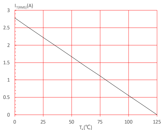
FIG.5: On-state characteristics
