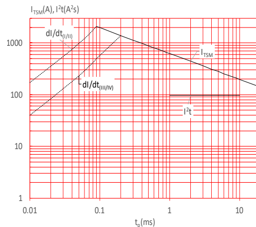
FIG.6: Non-repetitive surge peak on-state current for a sinusoidal pulse with width t_p < 20ms , and corresponding value of I^2t (I - II: di/dt < 50A/\mu s ; III-IV: di/dt < 20A/\mu s )
