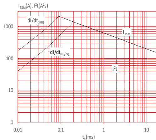
FIG.6: Non-repetitive surge peak on-state current for a sinusoidal pulse with width t_p < 20ms , and corresponding value of I^2t (I - II: di/dt < 80A/\mu s ; III-IV: di/dt < 50A/\mu s )
