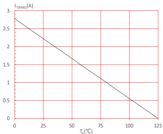
FIG.5: On-state characteristics
