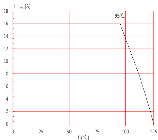
FIG.4: On-state characteristics
