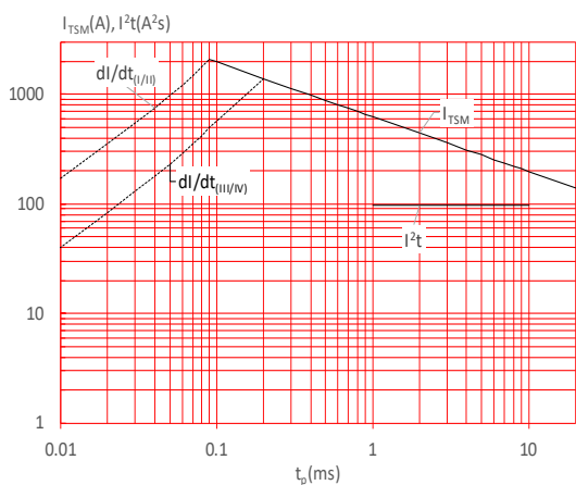
FIG.5: Non-repetitive surge peak on-state current for a sinusoidal pulse with width t_p < 20\text{ms} , and corresponding value of I^2t (I - II: di/dt < 80\text{A}/\mu\text{s} ; III-IV: di/dt < 50\text{A}/\mu\text{s} )
