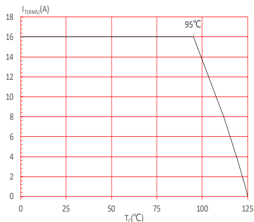
FIG.4: On-state characteristics
