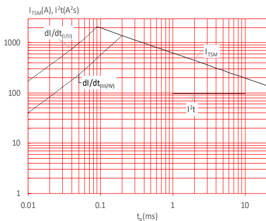
FIG.5: Non-repetitive surge peak on-state current for a sinusoidal pulse with width t_p < 20ms , and corresponding value of I^2t ( I - II: di/dt < 100A/\mu s; III - IV: di/dt < 70A/\mu s )
