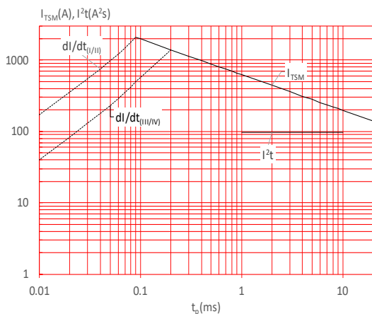
FIG.5: Non-repetitive surge peak on-state current for a sinusoidal pulse with width t_p < 20ms , and corresponding value of I^2t (I - II: di/dt < 80A/\mu s ; III-IV: di/dt < 50A/\mu s )
