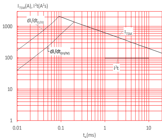
FIG.5: Non-repetitive surge peak on-state current for a sinusoidal pulse with width t_p < 20ms , and corresponding value of I^2t ( I - II : di/dt < 100A/\mu s ; III - IV : di/dt < 70A/\mu s )
