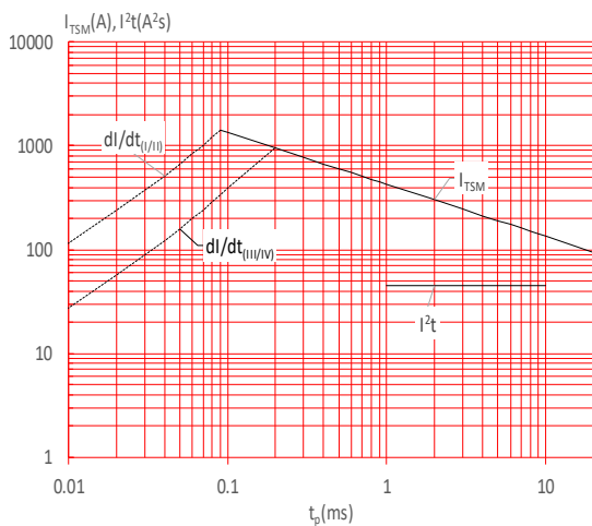
FIG.5: Non-repetitive surge peak on-state current for a sinusoidal pulse with width t_p < 20ms , and corresponding value of I^2t (I - II: di/dt < 80A/\mu s ; III-IV: di/dt < 50A/\mu s )
