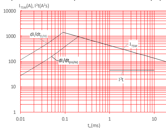
FIG.6: Non-repetitive surge peak on-state current for a sinusoidal pulse with width t_p < 20ms , and corresponding value of I^2t (I - II: di/dt < 80A/\mu s ; III-IV: di/dt < 50A/\mu s )
