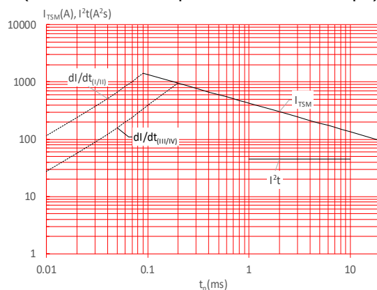
FIG.6: Non-repetitive surge peak on-state current for a sinusoidal pulse with width t_p < 20ms , and corresponding value of I^2t (I - II: di/dt < 100A/\mu s ; III-IV: di/dt < 70A/\mu s )
