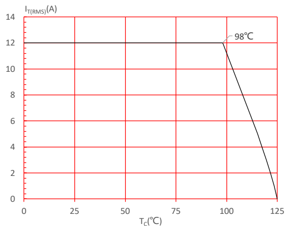
FIG.4: On-state character
