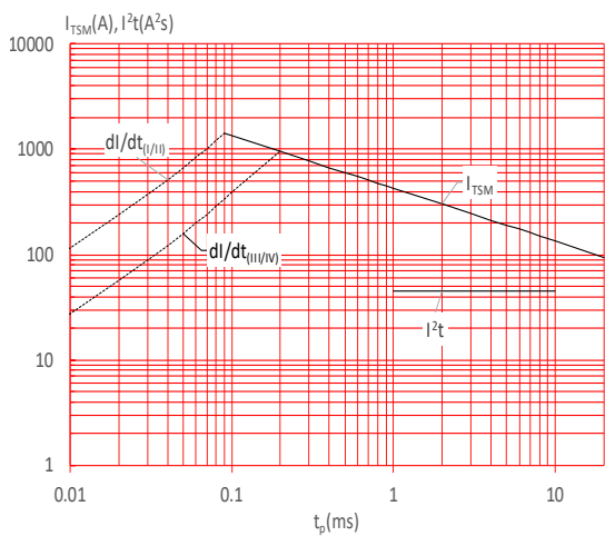
FIG.5: Non-repetitive surge peak on-state current for a sinusoidal pulse with width t_p < 20ms , and corresponding value of I^2t (I - II: di/dt < 50A/\mu s ; III-IV: di/dt < 20A/\mu s )
