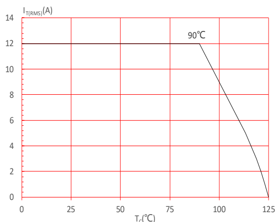
FIG.4: On-state character
