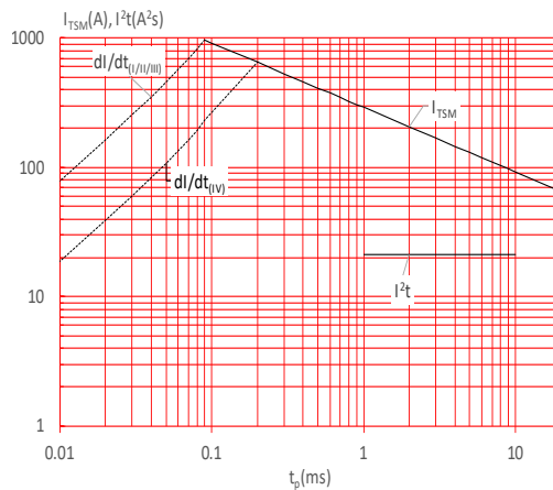
FIG.6: Non-repetitive surge peak on-state current for a sinusoidal pulse with width t_p < 20ms , and corresponding value of I^2t (I - II - III: di/dt < 100A/μs ; IV: di/dt < 50A/μs )
