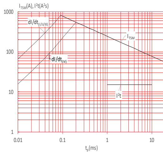
FIG.6: Non-repetitive surge peak on-state current for a sinusoidal pulse with width t_p < 20ms , and corresponding value of I^2t ( I - II - III: di/dt < 70A/\mu s ; IV: di/dt < 40A/\mu s )
