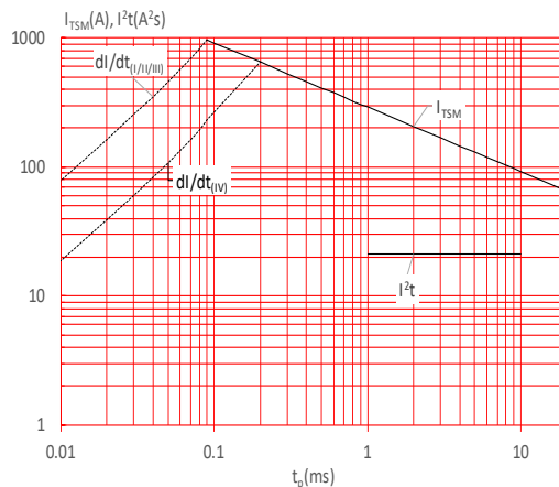
FIG.6: Non-repetitive surge peak on-state current for a sinusoidal pulse with width t_p < 20ms , and corresponding value of I^2t (I - II - III: di/dt < 100A/μs ; IV: di/dt < 50A/μs )
