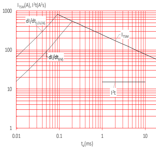
FIG.6: Non-repetitive surge peak on-state current for a sinusoidal pulse with width t_p < 20ms , and corresponding value of I^2t ( I - II - III: di/dt < 50A/\mu s ; IV: di/dt < 30A/\mu s )
