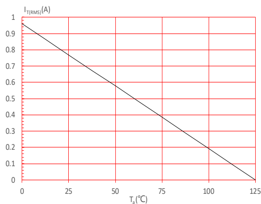
FIG.5: On-state characteristics
