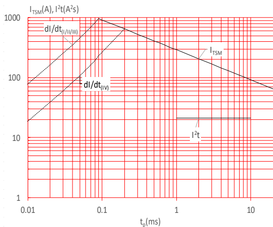
FIG.5: Non-repetitive surge peak on-state current for a sinusoidal pulse with width t_p < 20ms , and corresponding value of I^2t ( I - II -III: dl/dt < 100A/\mu s ; IV: dl/dt < 50A/\mu s )
