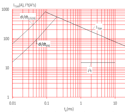
FIG.5: Non-repetitive surge peak on-state current for a sinusoidal pulse with width t_p < 20\text{ms} , and corresponding value of I^2t ( I - II - III: dl/dt < 70\text{A}/\mu\text{s} ; IV: dl/dt < 40\text{A}/\mu\text{s} )
