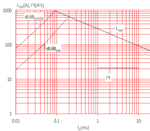
FIG.5: Non-repetitive surge peak on-state current for a sinusoidal pulse with width t_p < 20ms , and corresponding value of I^2t (I-II-III: dl/dt < 50A/\mu s ; IV: dl/dt < 20A/\mu s )
