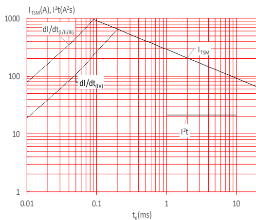
FIG.5: Non-repetitive surge peak on-state current for a sinusoidal pulse with width t_p < 20ms , and corresponding value of I^2t (I-II-III: di/dt < 100A/\mu s ; IV: di/dt < 50A/\mu s )
