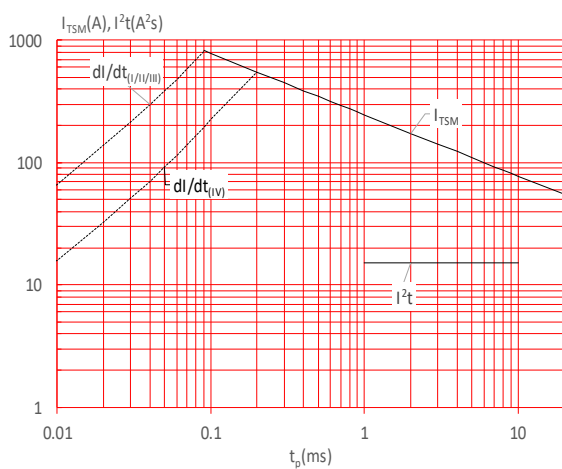
FIG.5: Non-repetitive surge peak on-state current for a sinusoidal pulse with width t_p < 20ms , and corresponding value of I^2t (I - II - III: di/dt < 50A/\mu s ; IV: di/dt < 30A/\mu s )
