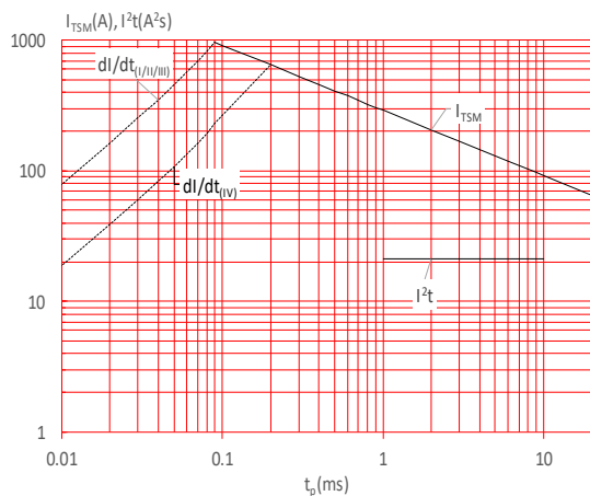
FIG.5: Non-repetitive surge peak on-state current for a sinusoidal pulse with width t_p < 20ms , and corresponding value of I^2t (I - II - III: dl/dt < 100A/\mu s ; IV: dl/dt < 50A/\mu s )
