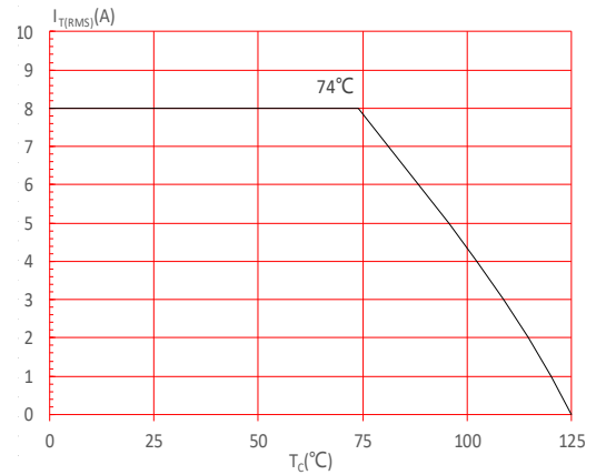
FIG.4: On-state characteristics
