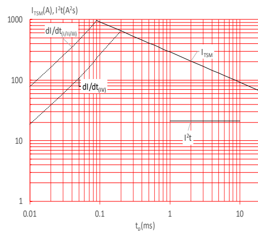
FIG.6: Non-repetitive surge peak on-state current for a sinusoidal pulse with width t_p < 20ms , and corresponding value of I^2t ( I - II - III: di/dt < 100A/\mu s ; IV: di/dt < 50A/\mu s )
