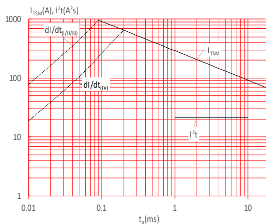
FIG.6: Non-repetitive surge peak on-state current for a sinusoidal pulse with width t_p < 20 ms, and corresponding value of I^2t (I - II - III: di/dt < 100 A/ \mu s; IV: di/dt < 50 A/ \mu s)
